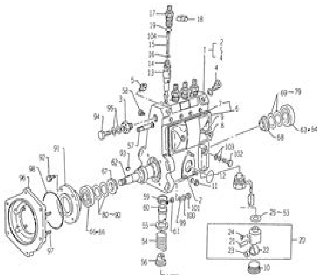
FIG. 16 COMPONENT PARTS FOR 6894 - 476 - 121 - 10 6897 - 030 - 187 - 00 ON Fig.14
