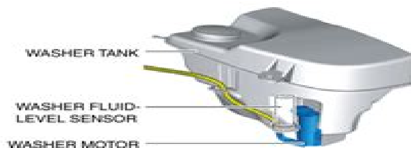
WITH WASHER FLUID-LEVEL SENSOR
