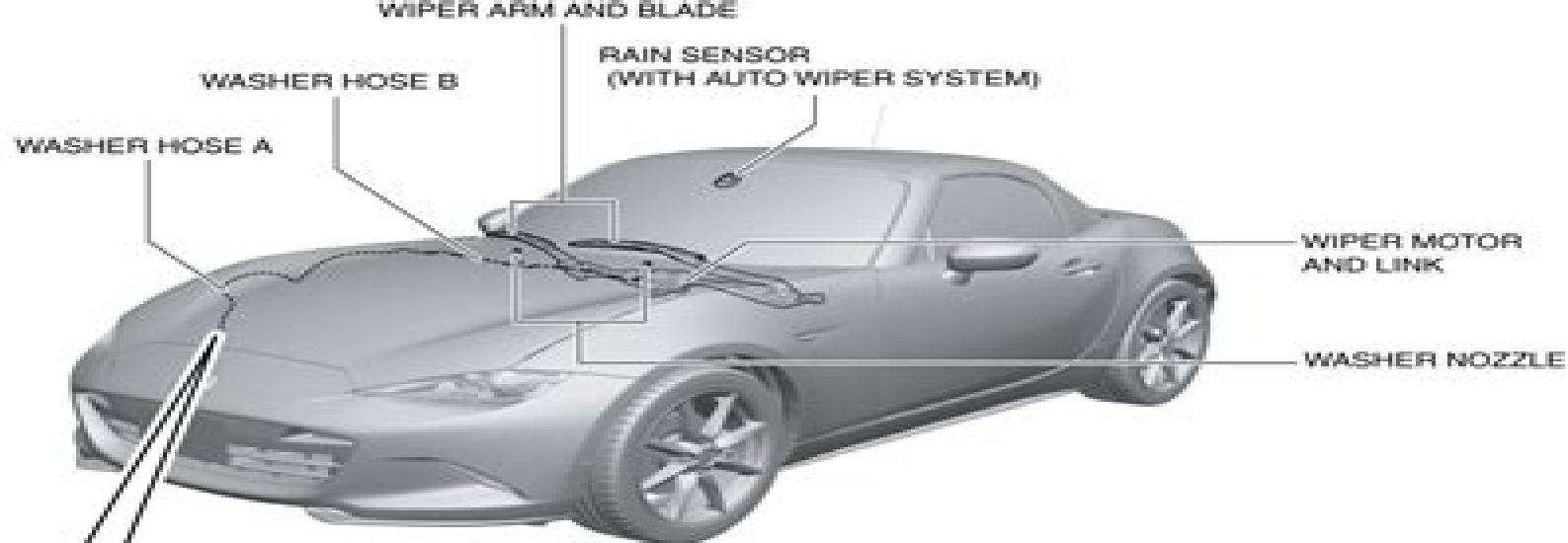
WITHOUT WASHER FLUID-LEVEL SENSOR
