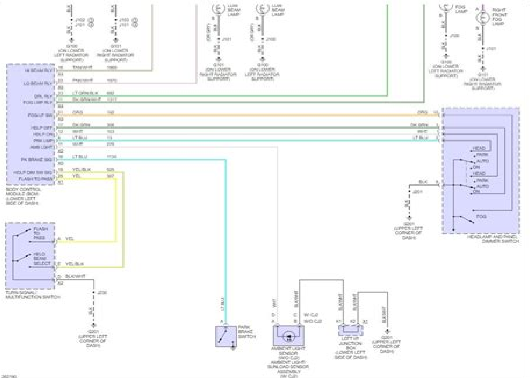
Fig 1: Headlights Circuit
