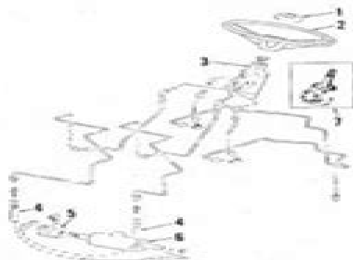
Fig. 3—Schematic view showing general layout of component parts of typical power steering system on International tractors. Hand pump and steering valve (3) is used on Models 434, 454, 574 and 574. Daneless pump and steering valve (7) is used on Models 484 and 584.
