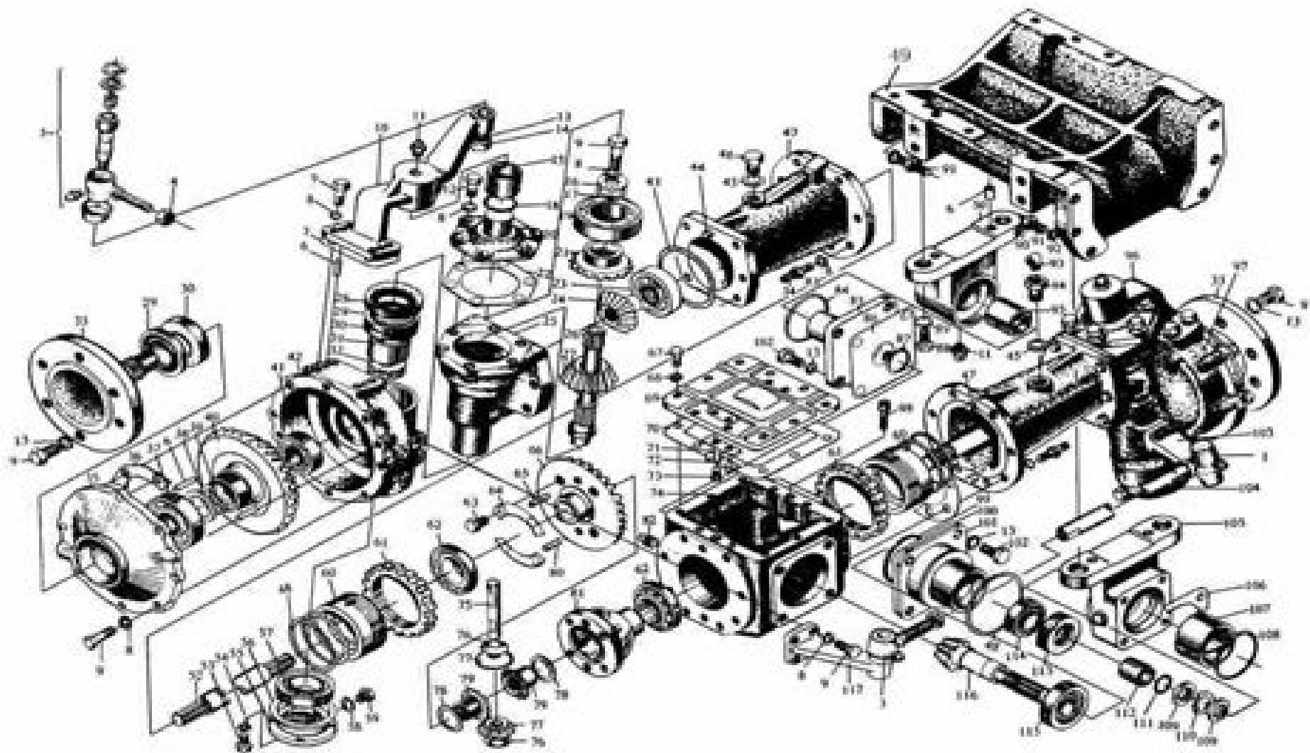
Fig. 3-A Front Axle For Hydraulic Steering
