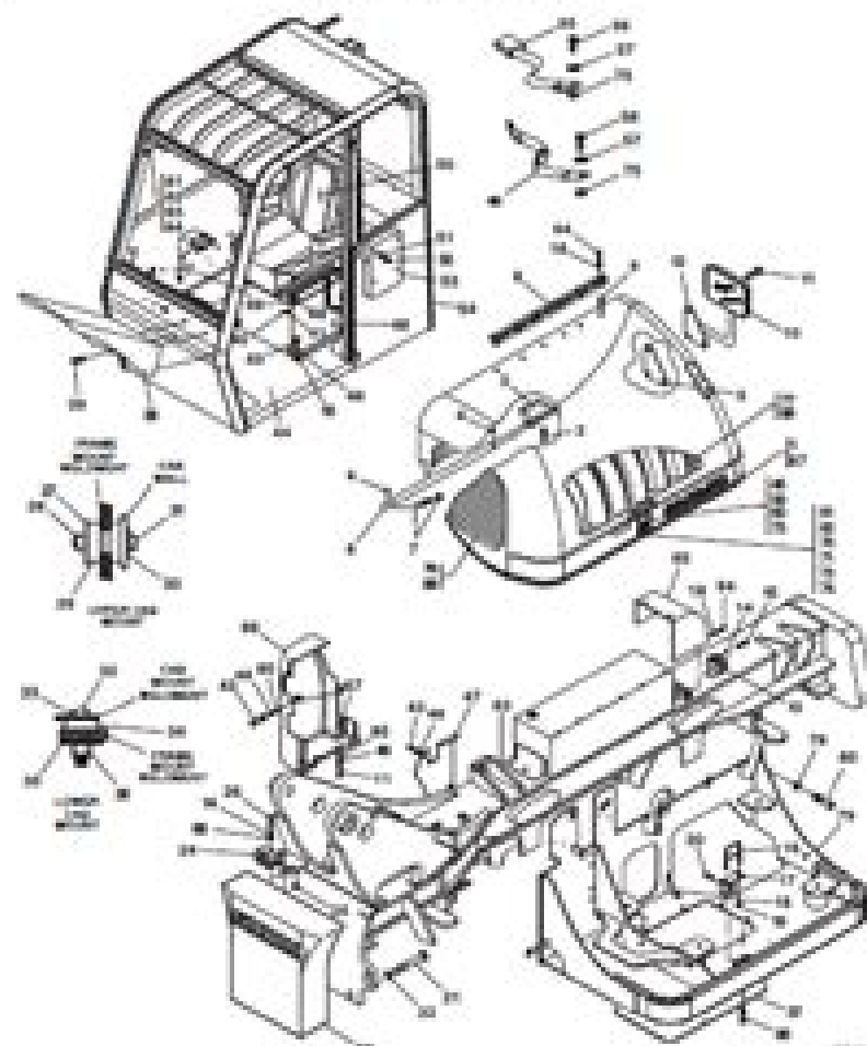
Figure 1-1 Frame Structure &amp; View
