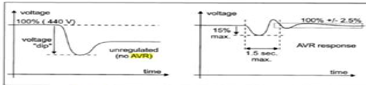
Fig. 3.11 Generator AVR voltage response.
