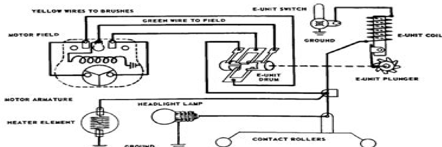
SCHEMATIC WIRING DIAGRAM OF NO. 736 LOCOMOTIVE
