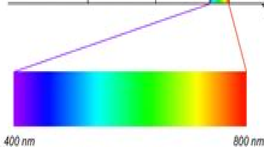
Spectre visible
