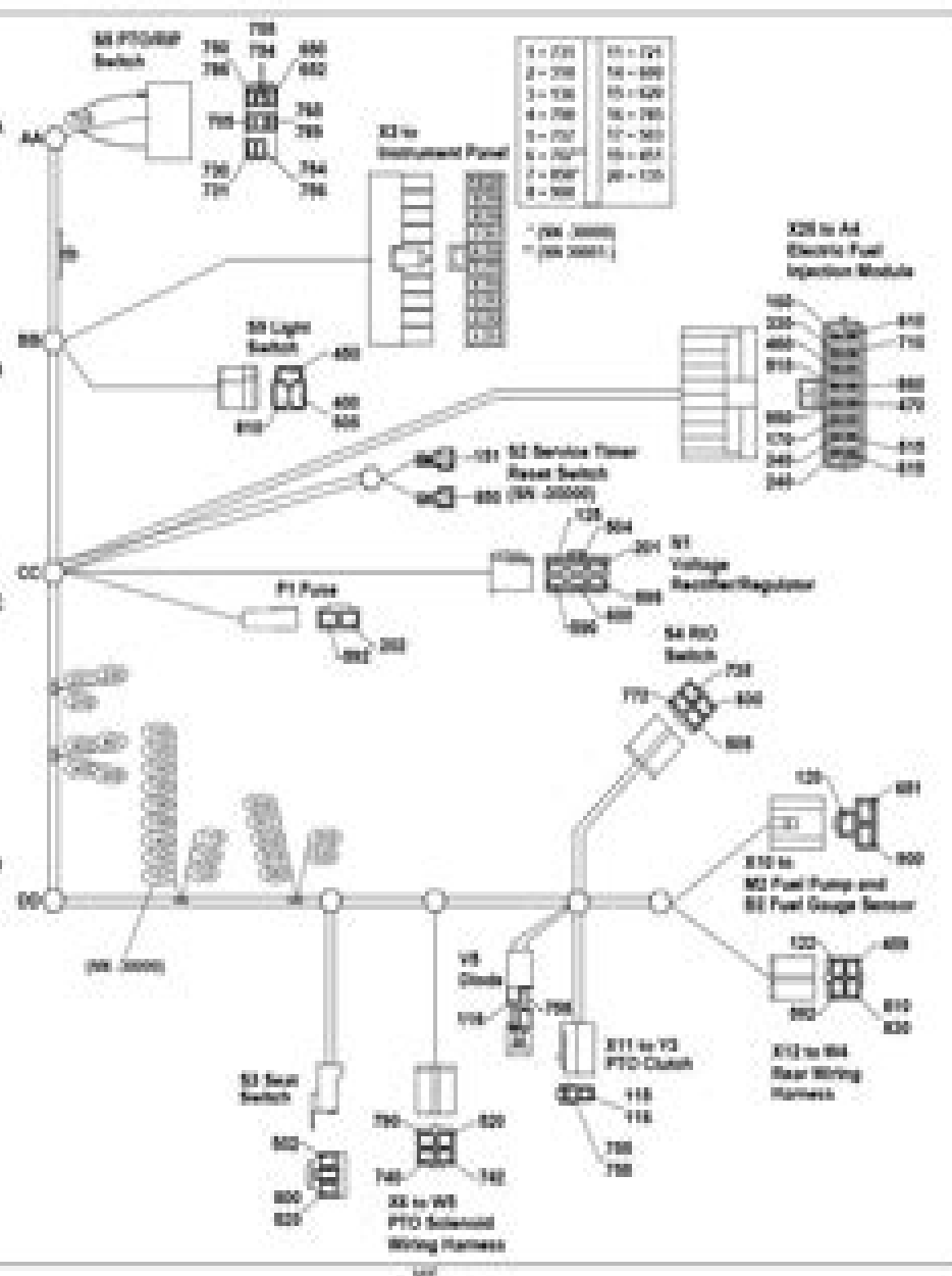
1 Main Wiring Harness - X485 and X585 (2 of 2)
