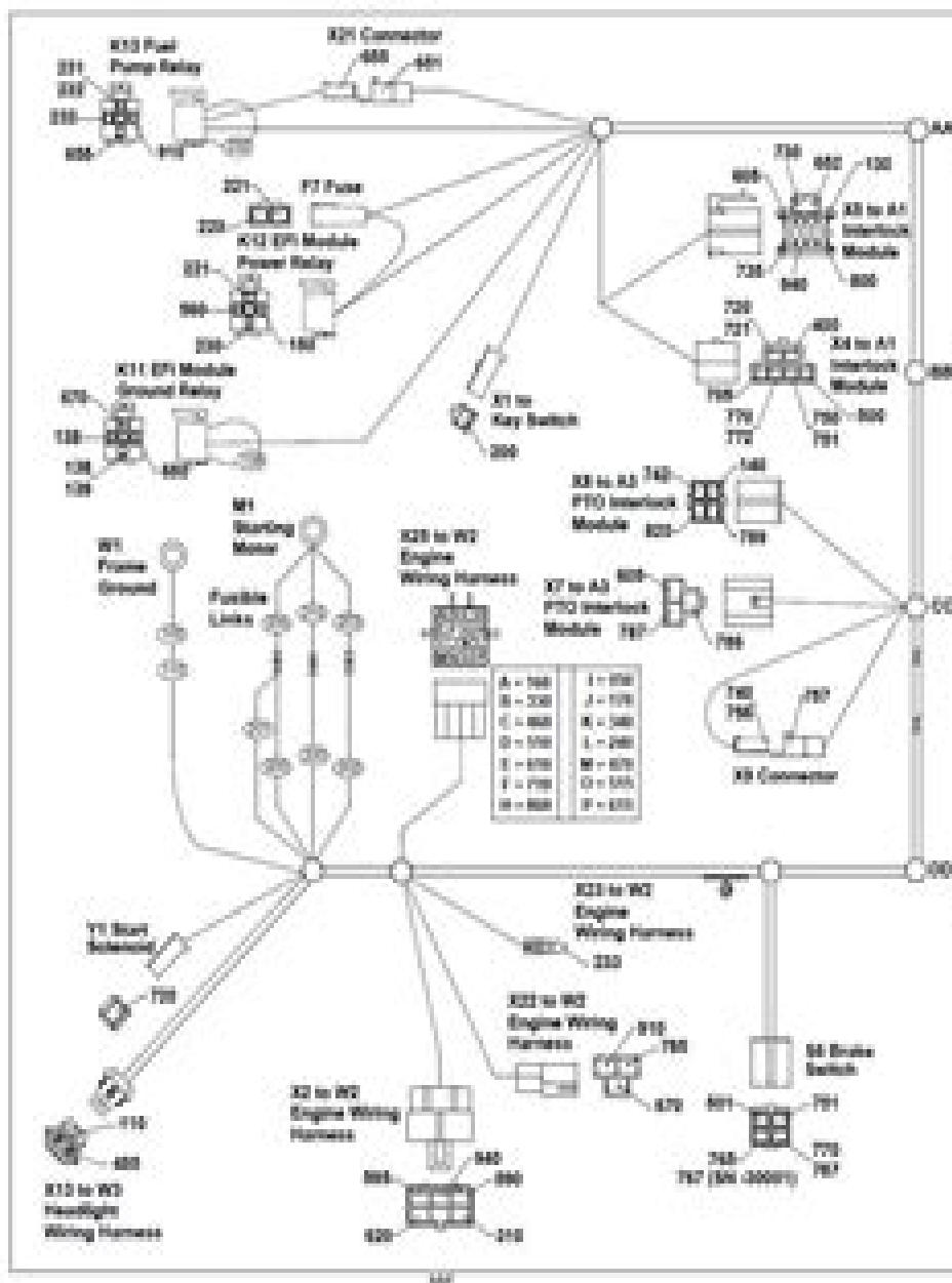
W1 Main Wiring Harness - X485 and X585 (1 of 2)
