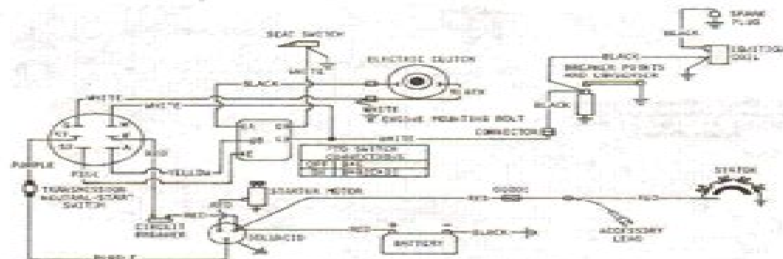
Fig. 4D107—Electrical wiring diagram for Models 108 and 111 tractors (S.N. 95001-120000).
