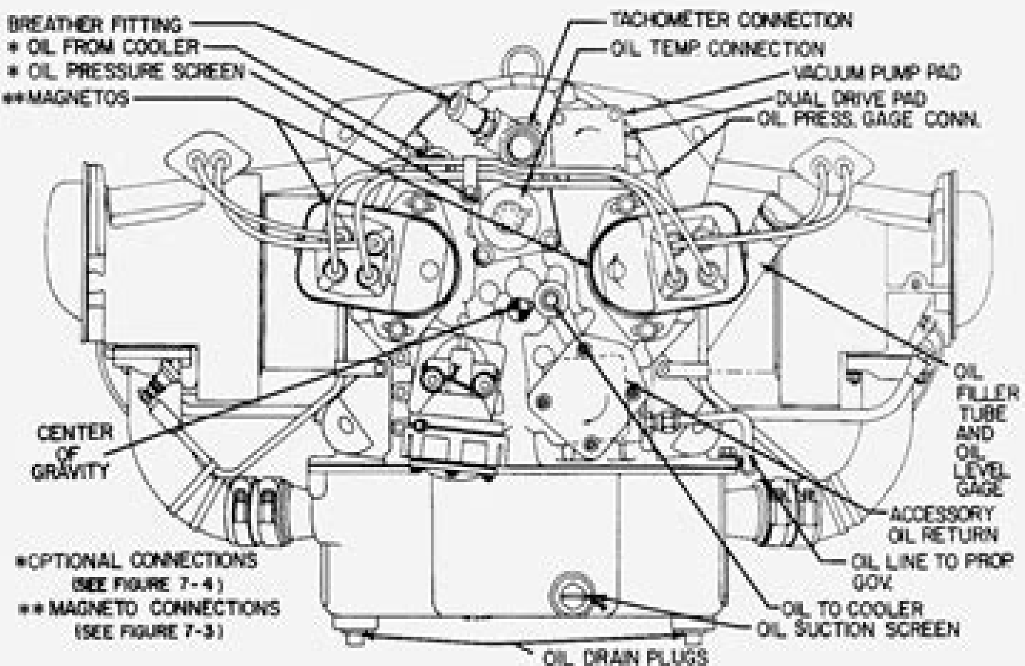
Figure 7-8. Installation Drawing Rear View - Typical O-320-D, -E Series
