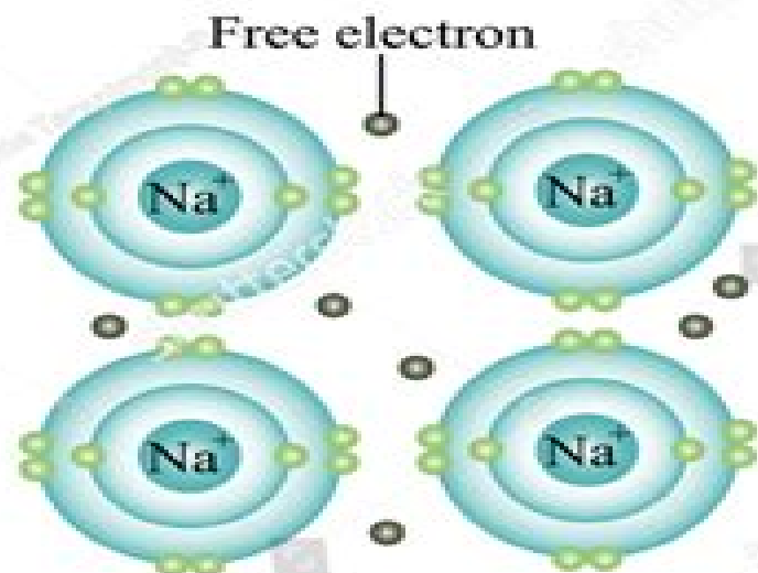
Metallic Bonding
