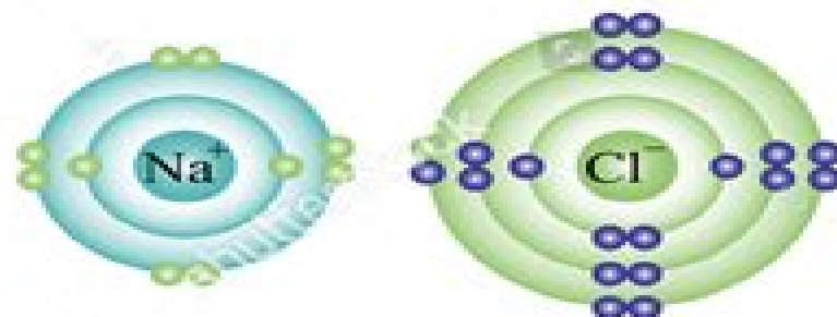
Ionic Bonding
