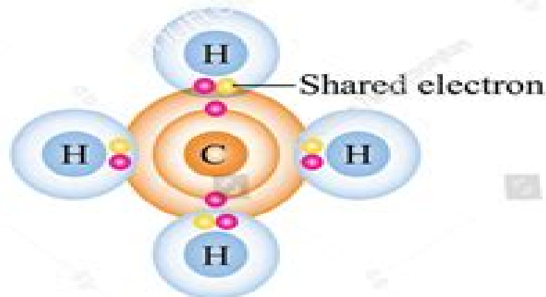
Covalent Bonding
