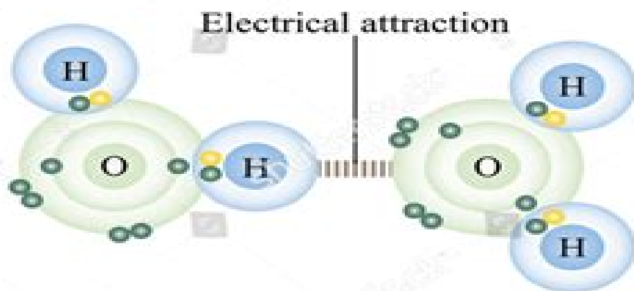
Molecular Bonding
