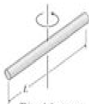
Thin rod about center I = \frac{1}{12} ML^2
