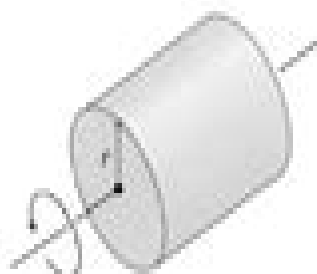
Disk or solid cylinder about its axis I = \frac{1}{2} MR^2
