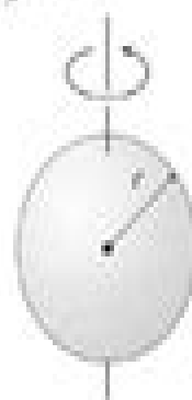
Solid sphere about diameter I = \frac{2}{5} MR^2
