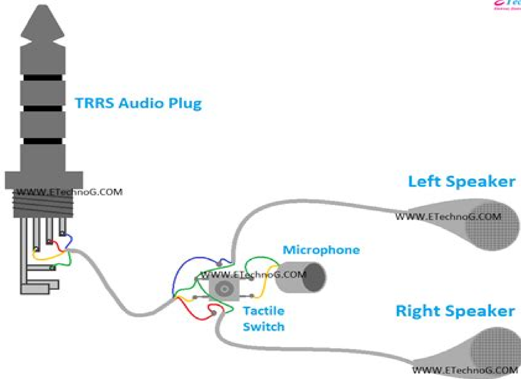
Stereo Headphone Jack Wiring and Connection Diagram
