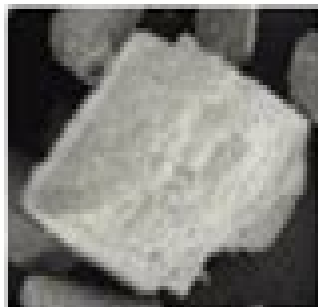
Equant particle
