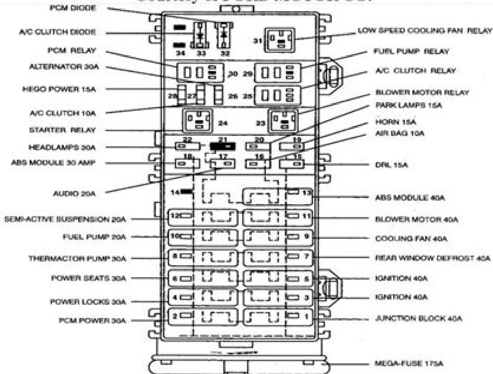
Fig. 6: Identifying Battery Junction Box Components
