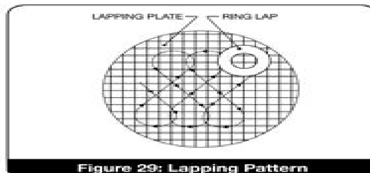
Figure 29: Lapping Pattern
