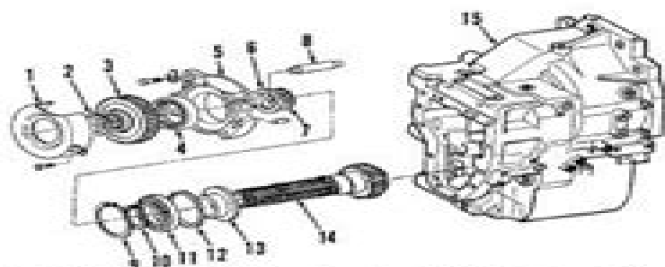
Fig. 138—Exploded view of mechanical front-wheel drive intermediate drive shaft and gear used on models equipped with Quad-Range transmission.
