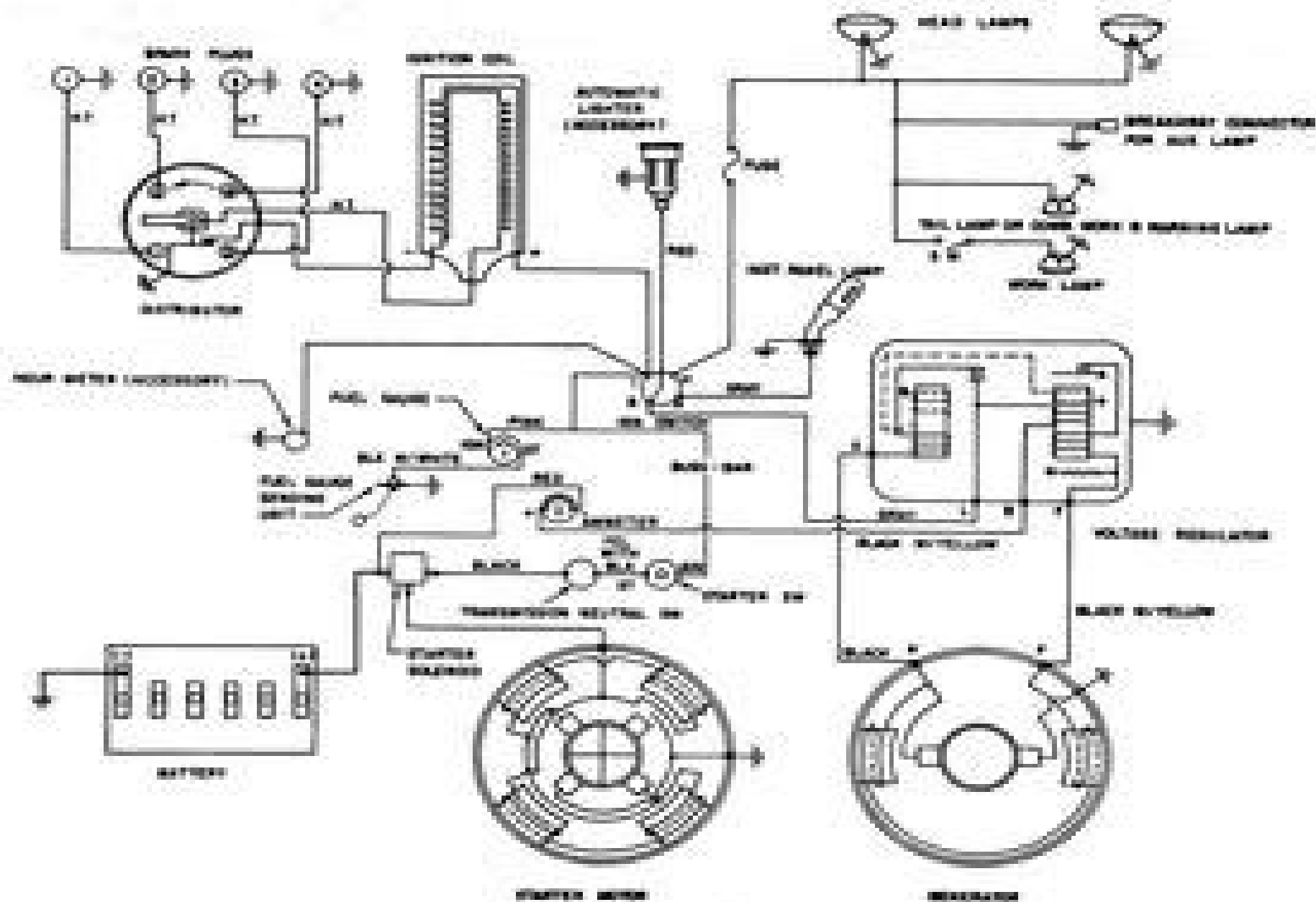
Fig. 30 - Electrical System - Gasoline
