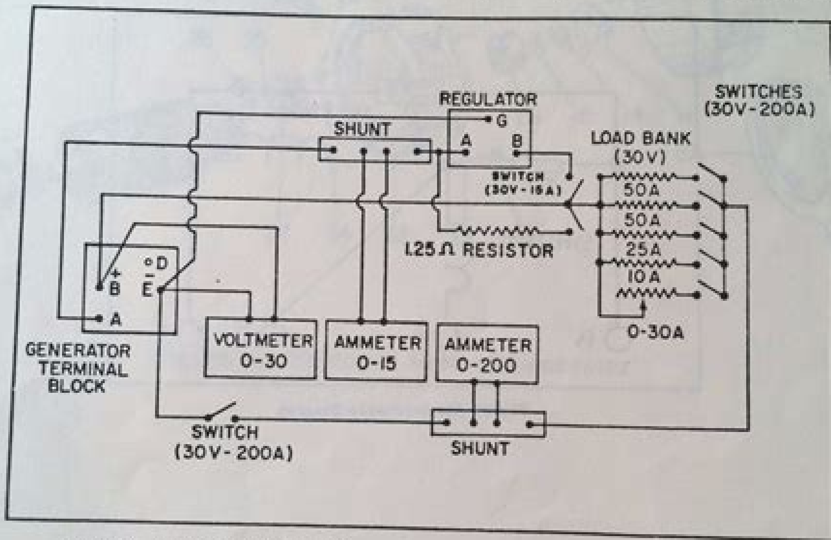
Figure 3. Diagram of Circuit Connections for Generator Performance Test
