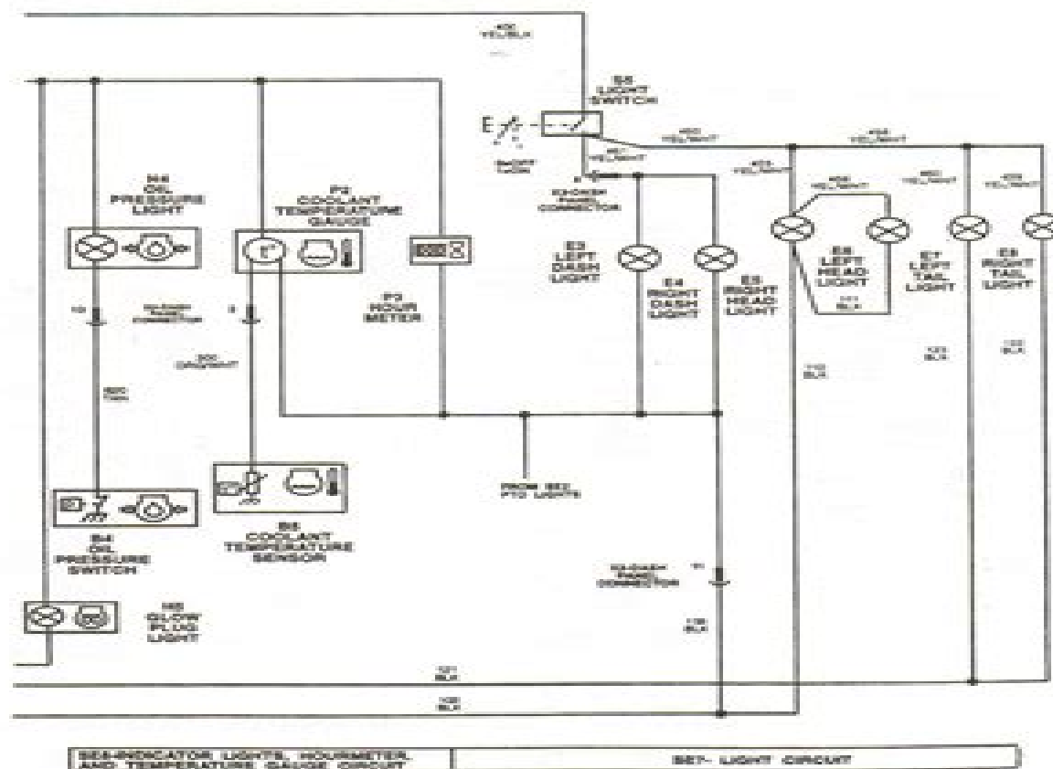
Fig. JDT-F1C—Partial wiring schematic for Model 455.
