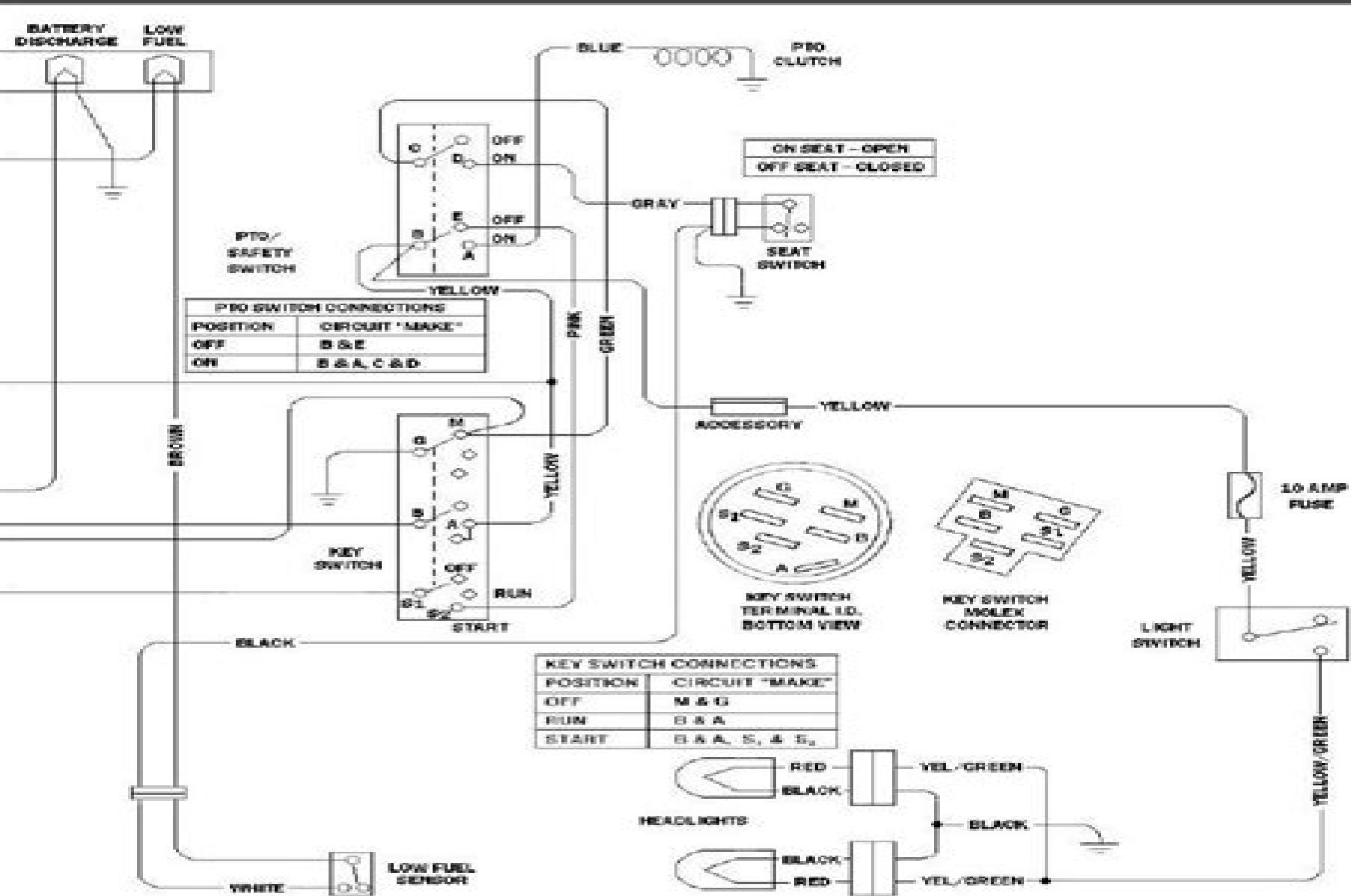
WIRING SCHEMATIC - 180 AND 185 TRACTORS (S.N. - 475000 ORS)
