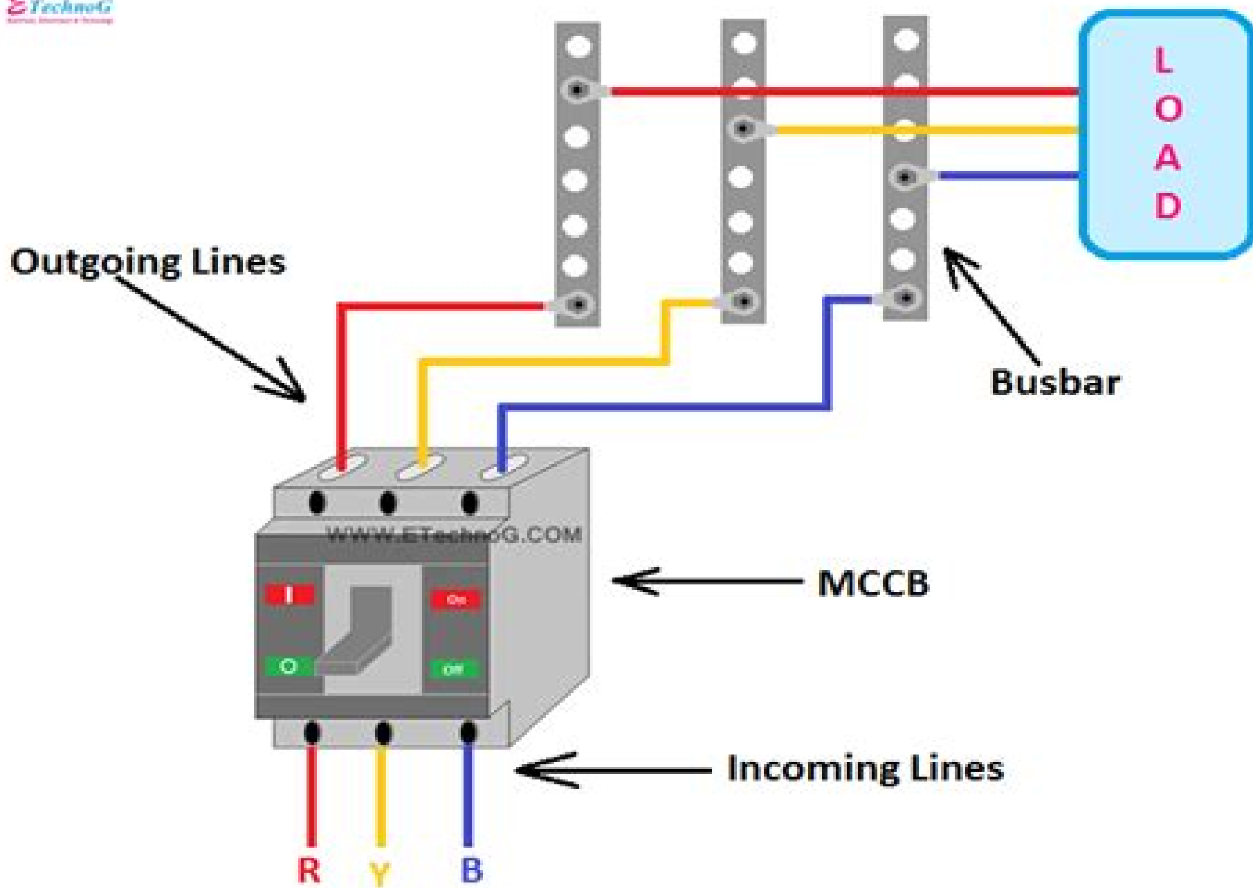
Three(3) Pole MCCB Wiring Connection
