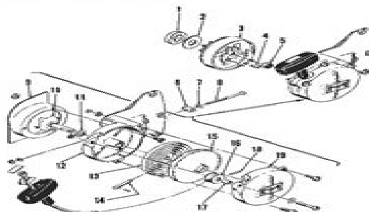
Fig. MC5-26—View showing disassembly of clutch and starter assemblies used on Models 725, 797 and Super 797.
