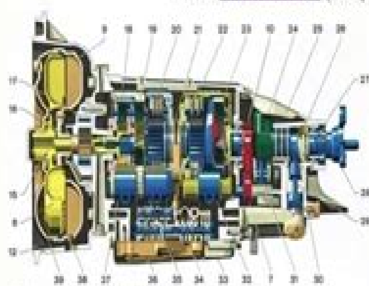
Fig. 1 4-speed transmission with fluid coupling
