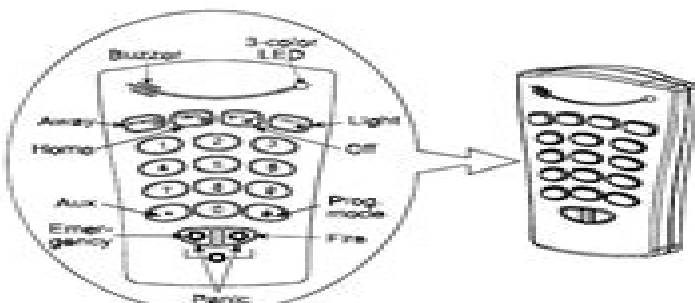
Figure 1 - External View
