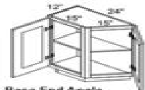
Base End Angle BEA1224 Interchangeable L & R Note - Same doors as W1530
