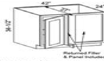
Base Blind Corner BBC42 - Interchangeable L & R Resize to BBC45 by + WDR19.5x30 Resize to BBC48 by + WDR21.5x30
