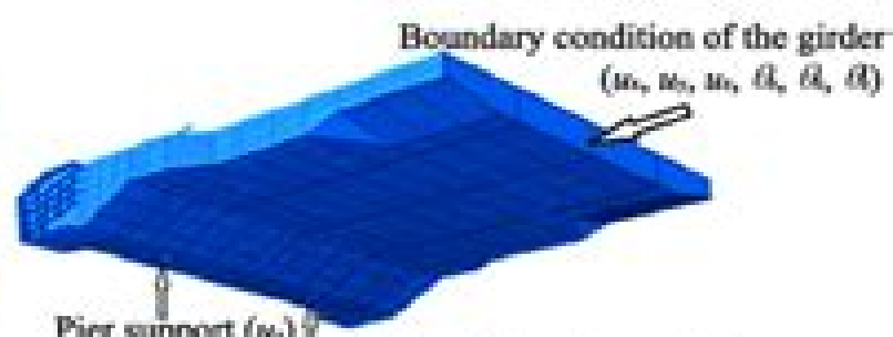
(c) Boundary condition(full-scale model)
