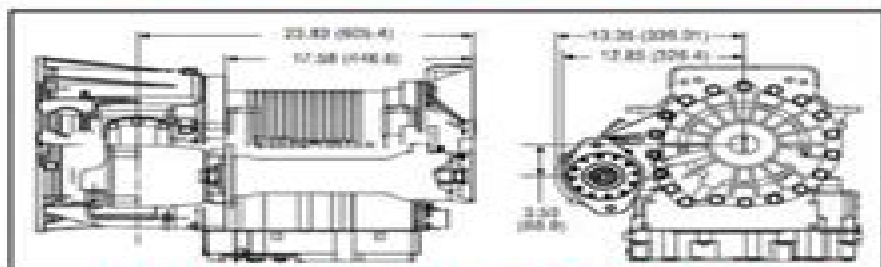
CS10 W/SHAFT EXTENSION
