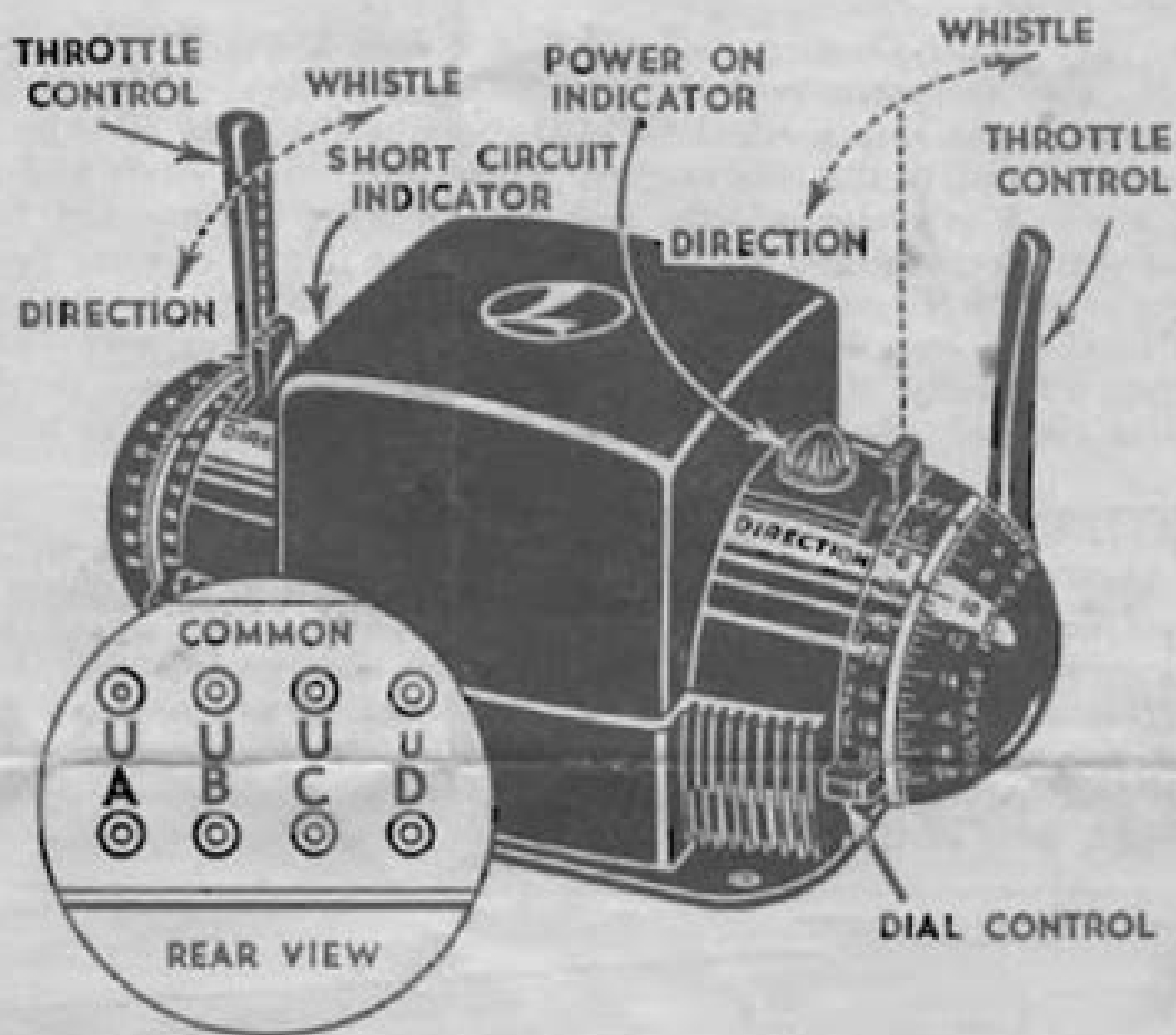
Figure 1—Type ZW "Multi-Control" Transformer.
