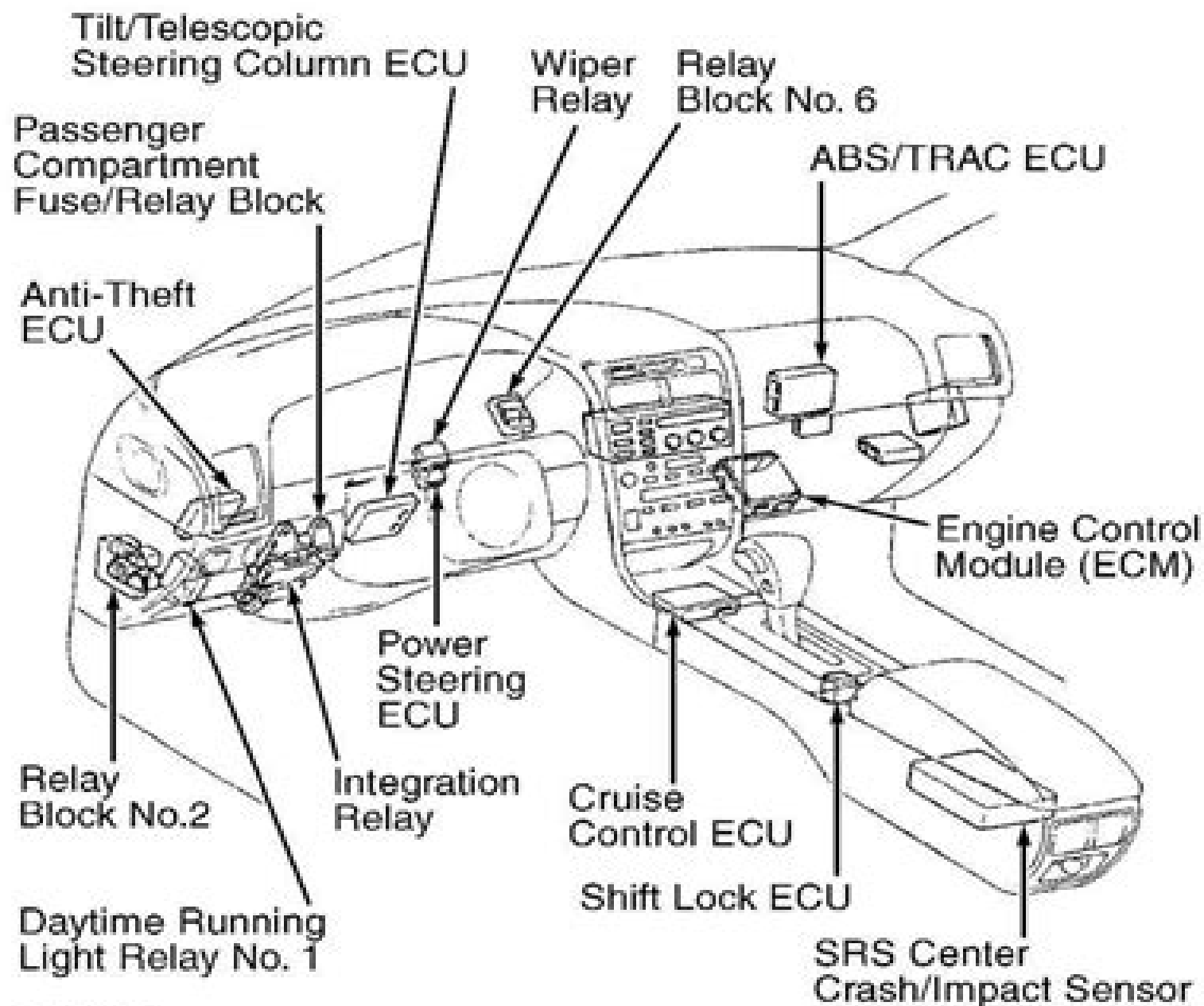
Fig. 1: Component Locations (1 Of 3)
