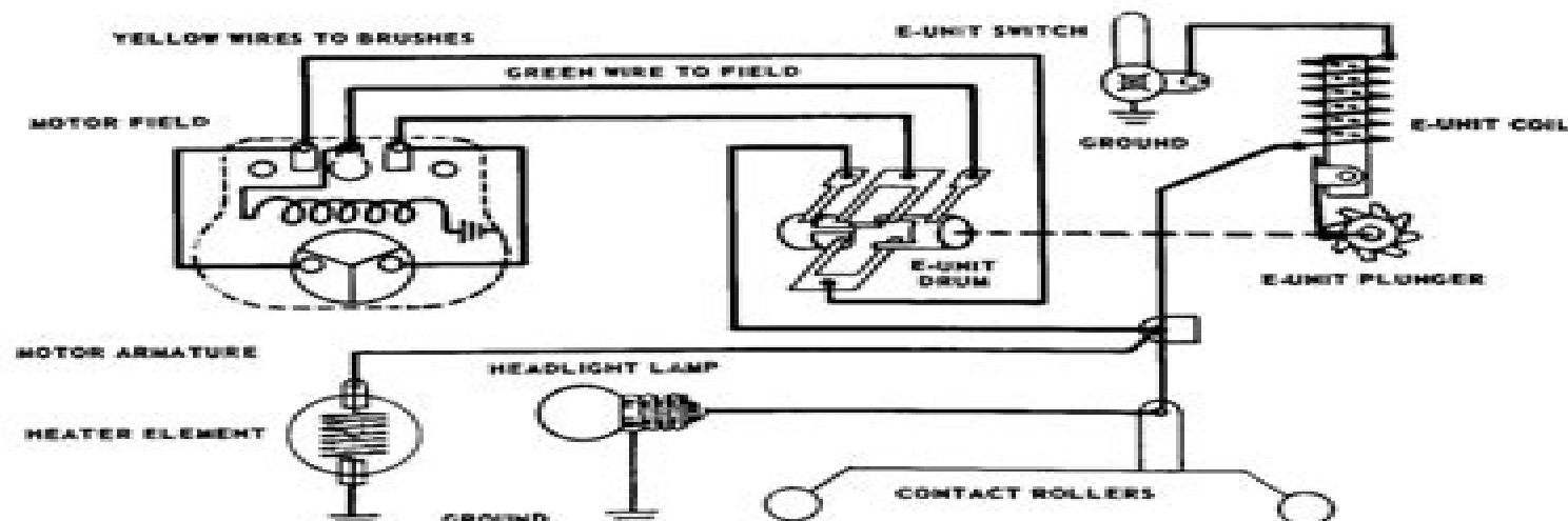
SCHEMATIC WIRING DIAGRAM OF NO. 736 LOCOMOTIVE
