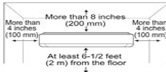
Figure 12: Single Zone Extended Piping Wall Mount Indoor Unit Clearance Requirements.
