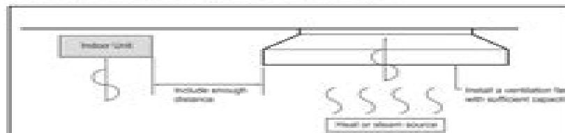
Figure 11: Installing Near a Heat or Steam Source.
