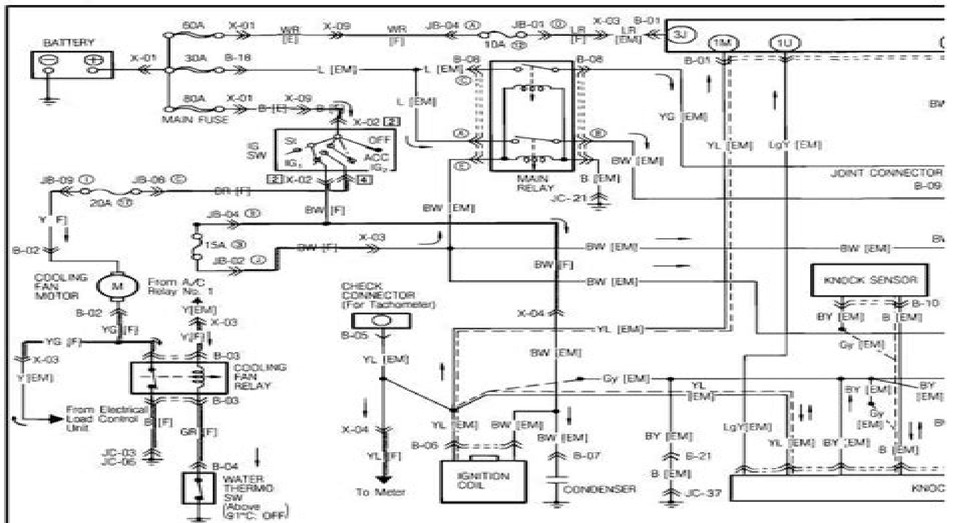
B-01 Engine Control Unit [EM]
