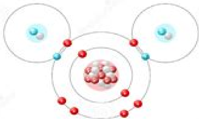
Covalent bond
