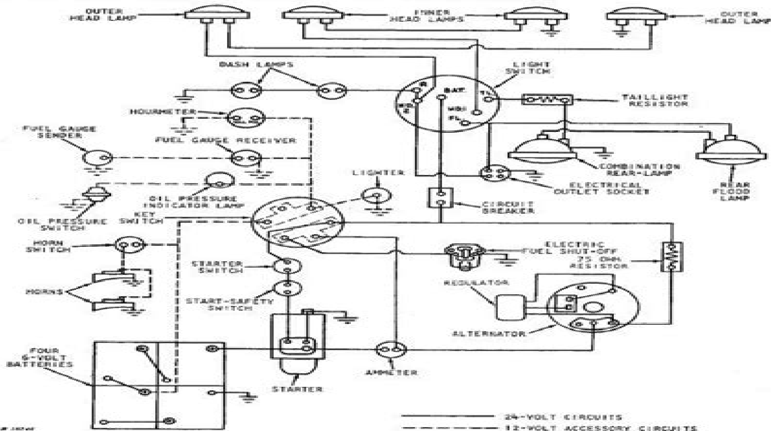
Fig. 150-10-1—Schematic Diagram of the Electrical System
