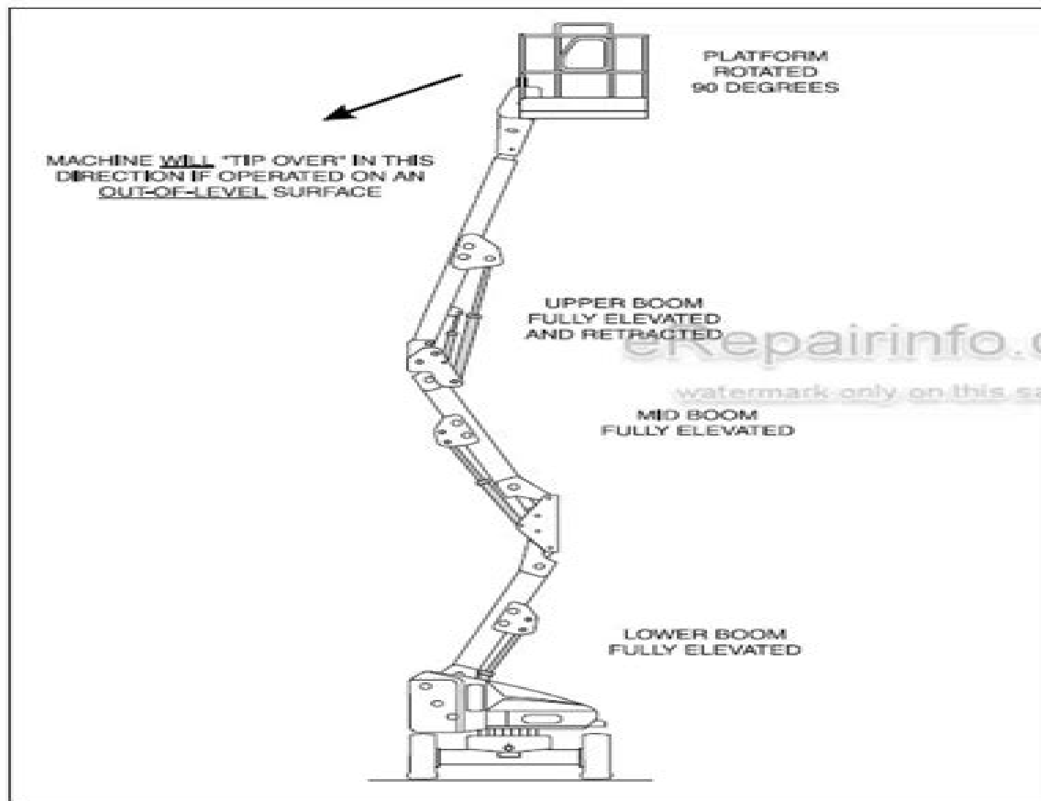
Figure 3-2. Position of Least Backward Stability
