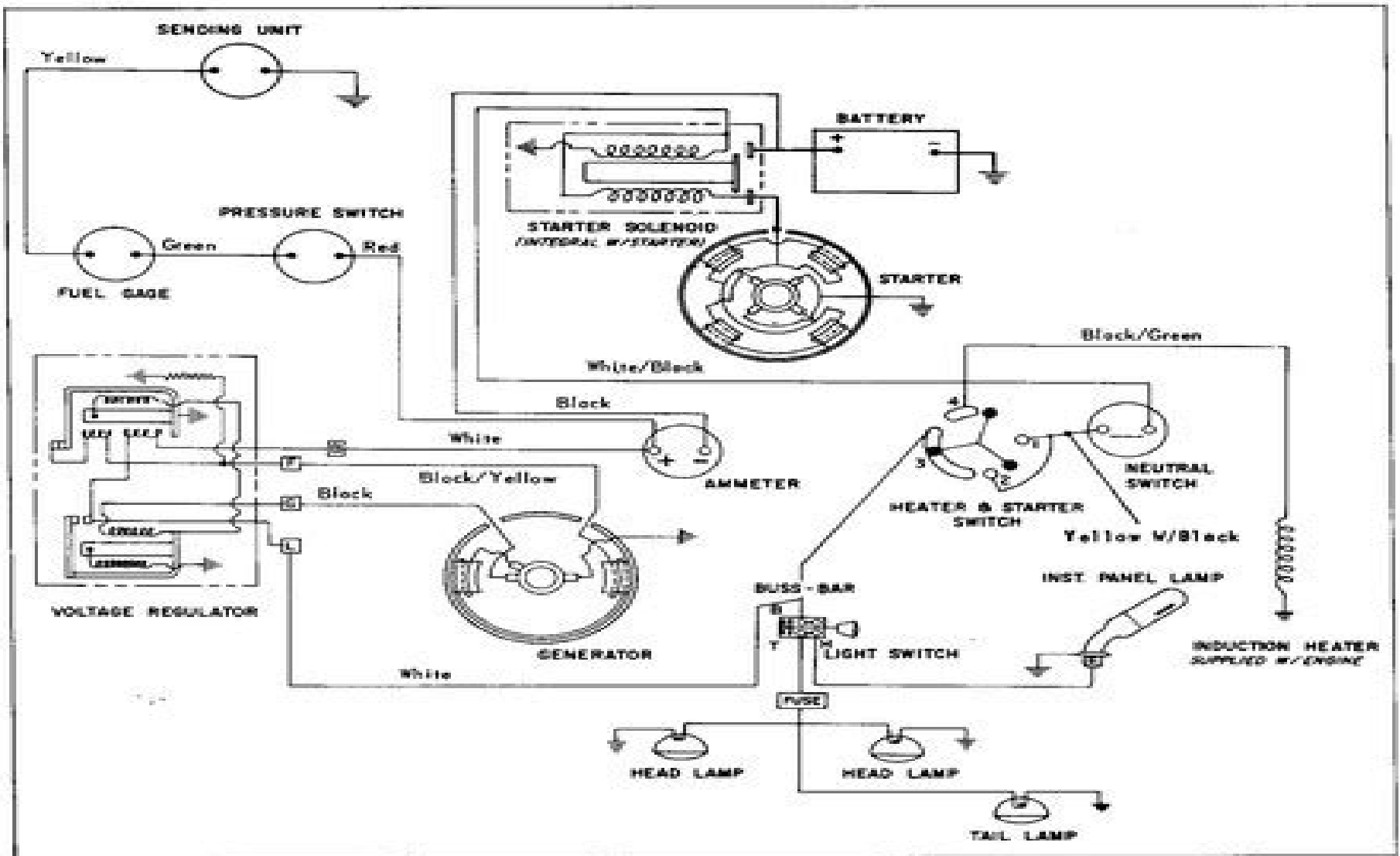
Electrical System (Diesel Tractors)
