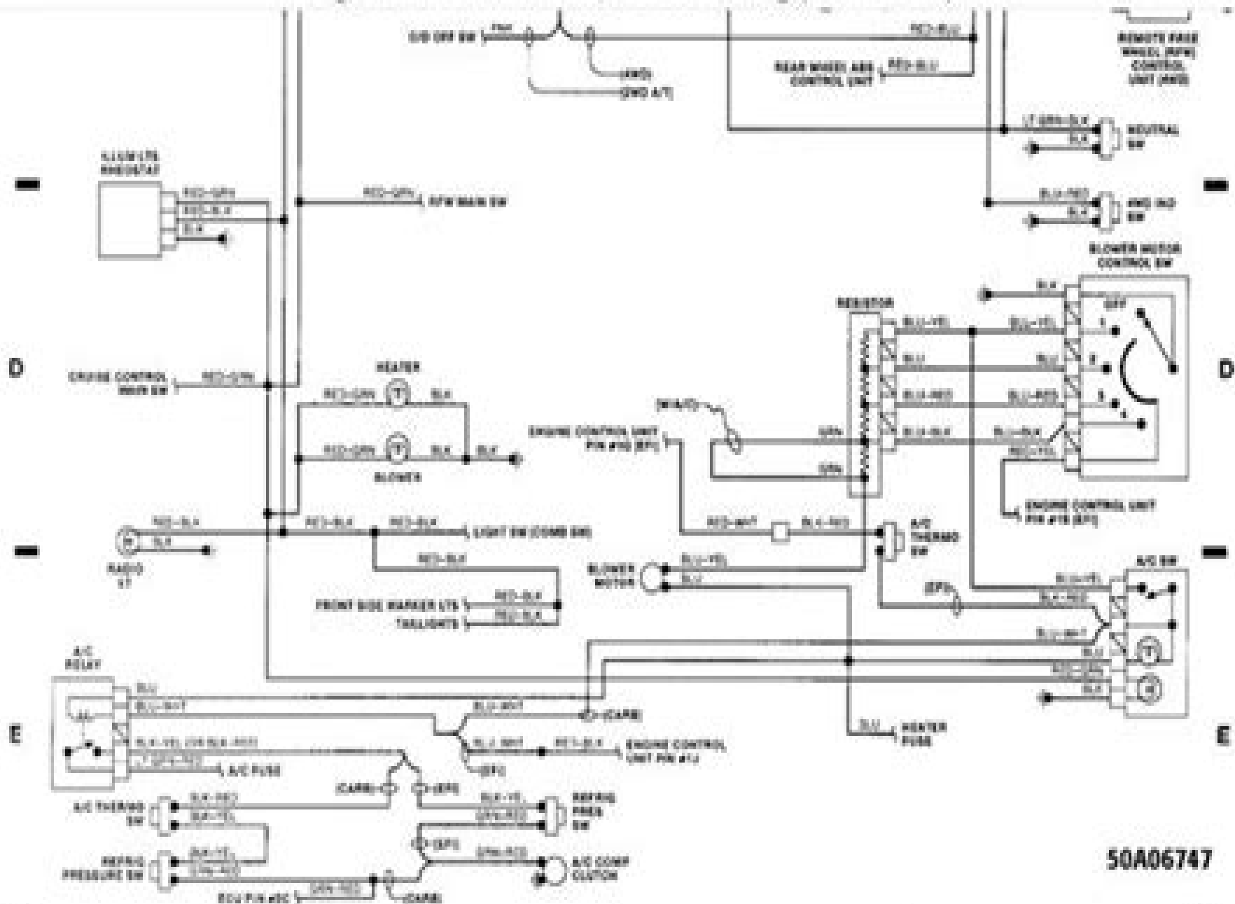
Fig. 5: Instrument Panel, A/C & Heating (Grids 16-19)
