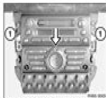
Fig. 1. Radio Receiver Mounting Screws And Removal Direction Courtesy of BMW OF NORTH AMERICA, INC.
