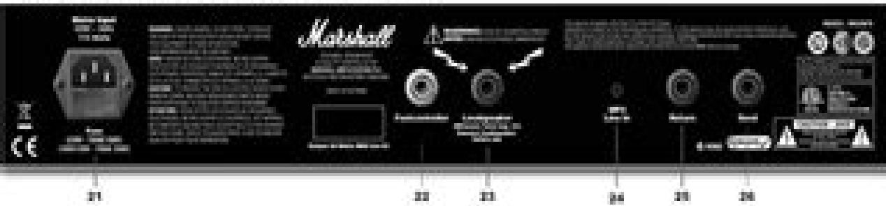
Head panel shows MG50FX combo - MG100FX combo has the same features MG100FX head is identical except features two footpedal sockets
