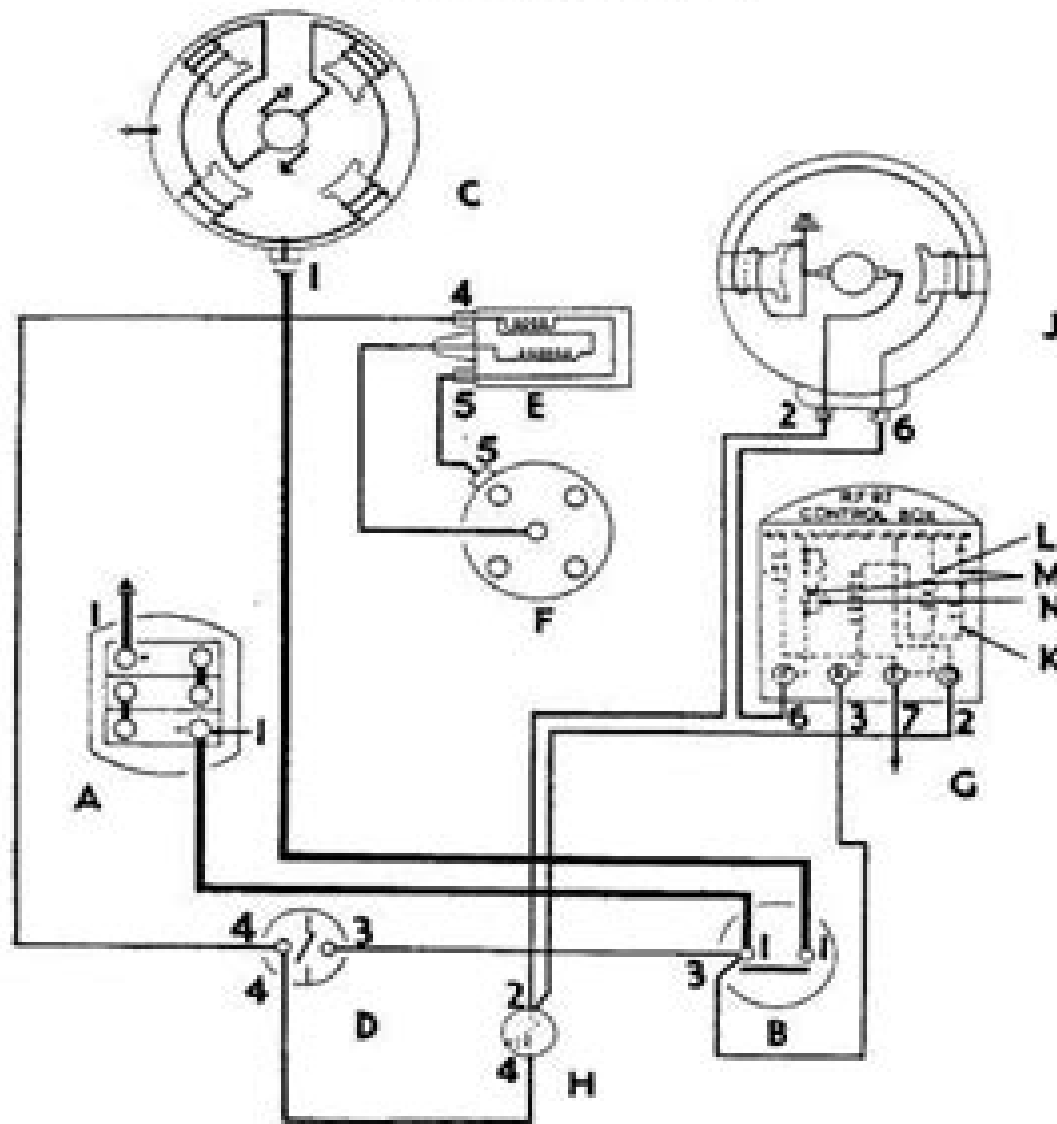
TRACTOR WIRING DIAGRAM.
