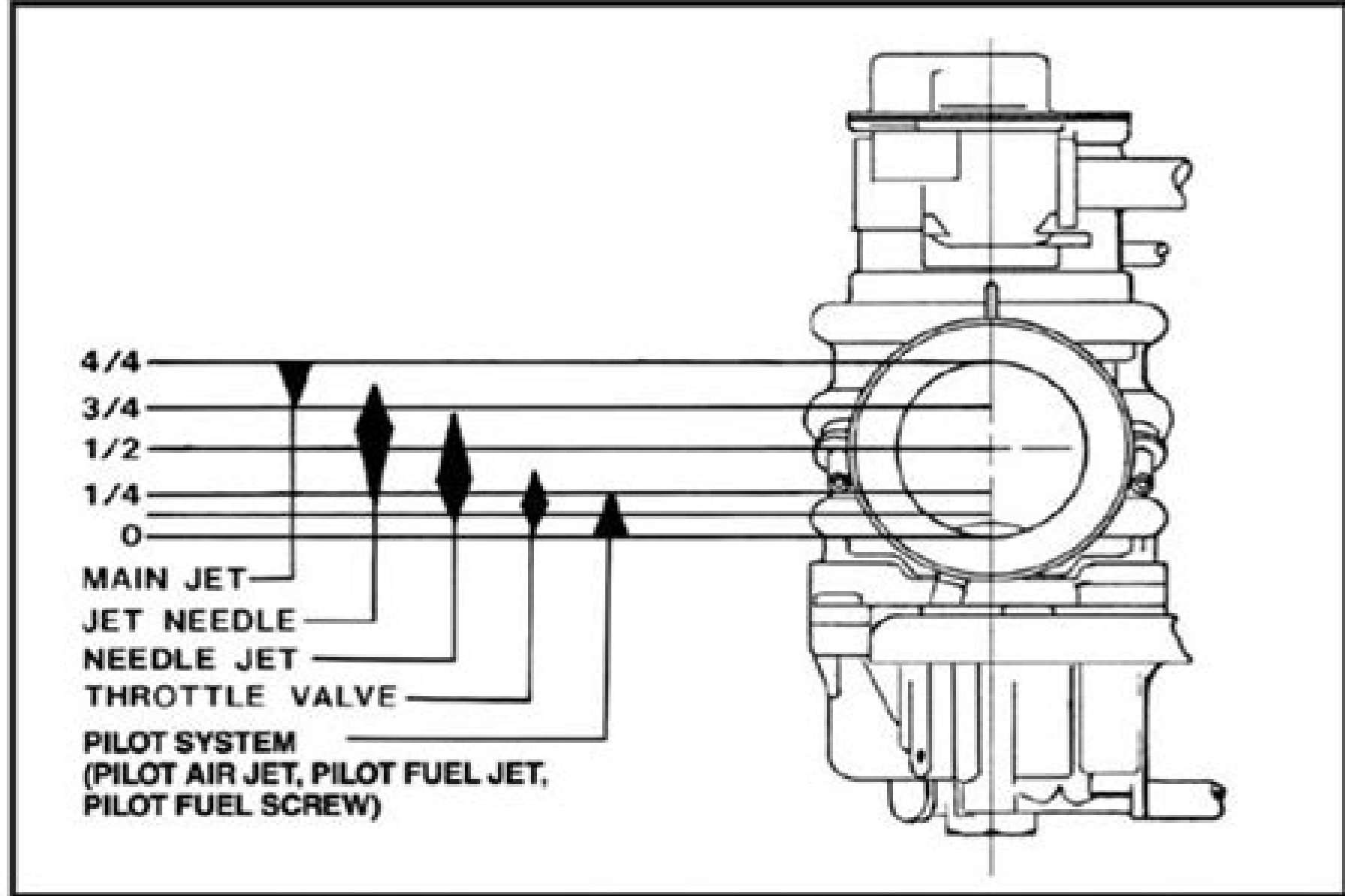
Diagram showing the effective range of the each tuning component of the Mikuni HS40 carburetor
