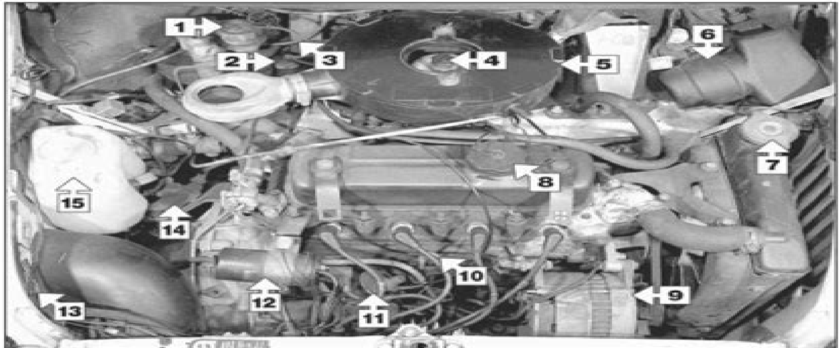
Underbonnet view of a 998 cc Mini 1000 Saloon
