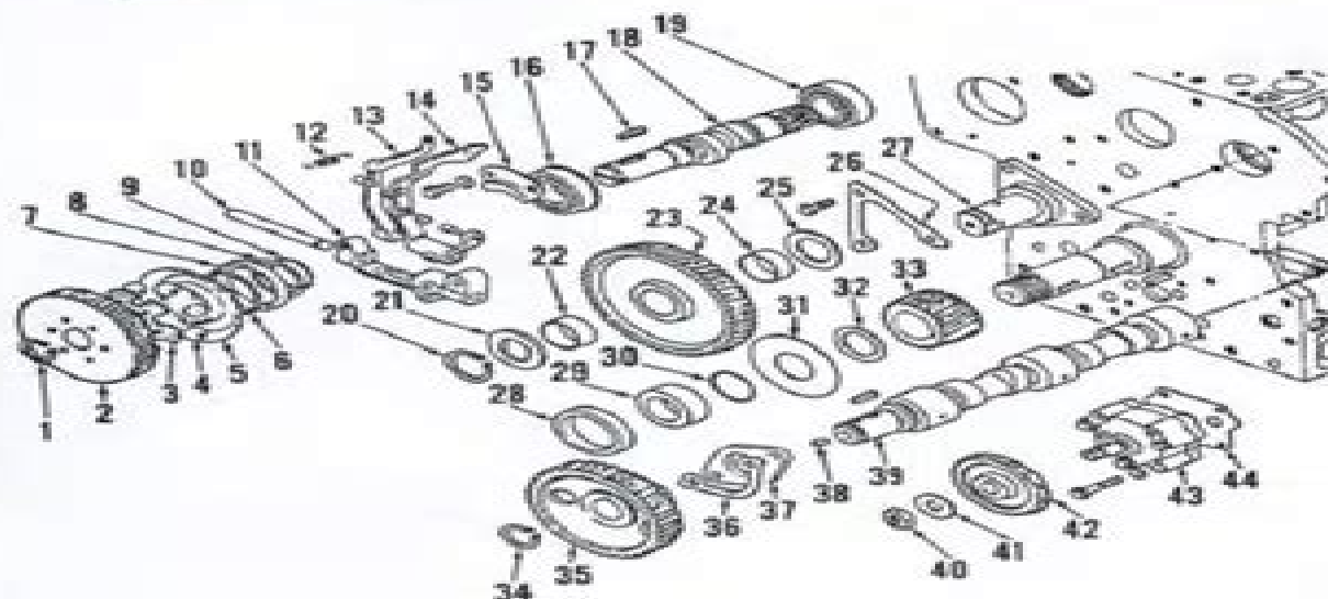
Fig. 25—Exploded view of timing gears and associated parts used on Models L175, L225 and L225DT.
