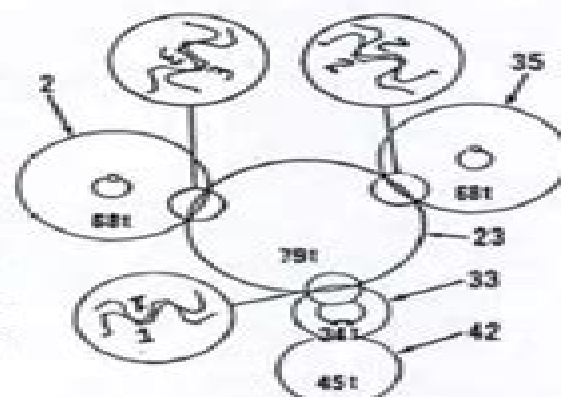
Fig. 26—Schematic view of timing gears on Models L175, L225 and L225DT showing timing marks. Refer to legend in Fig. 25 for identification of gears.
