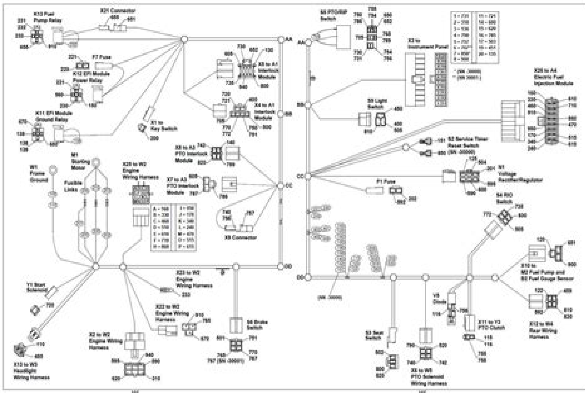
W1 Main Wiring Harness - X485 and X585 (1 of 2)
