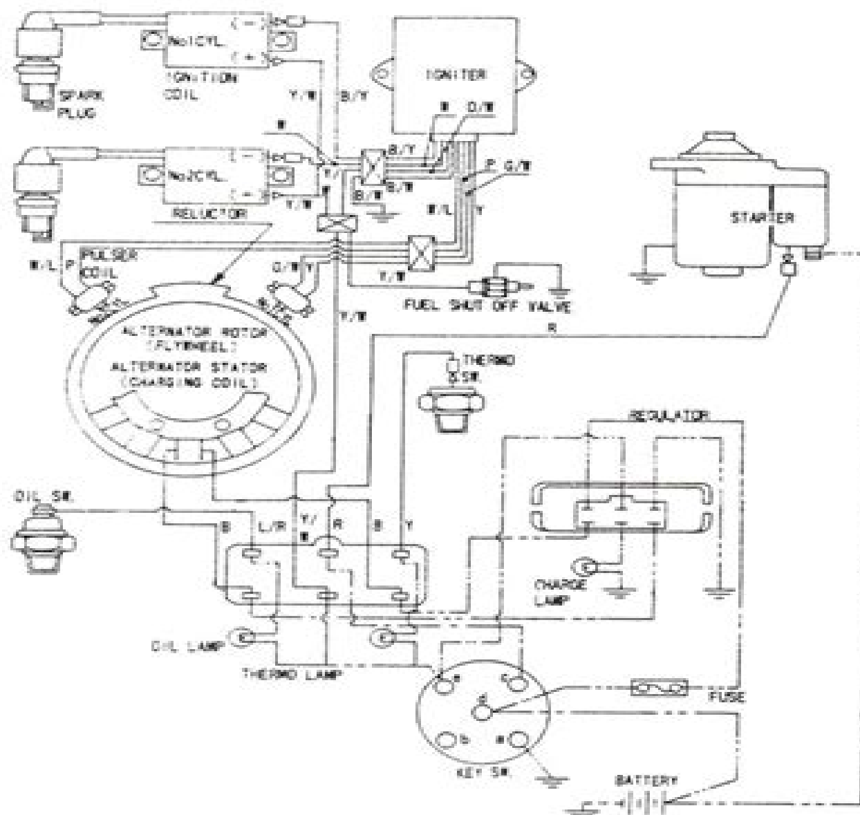
K518-Engine wiring diagram.
