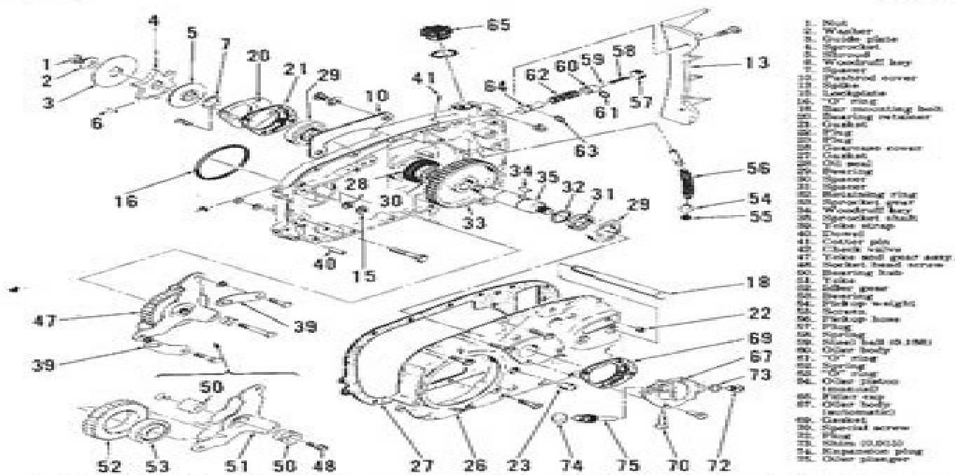
Fig. MCS-24—Exploded view of transmission gear used on Models 895 and 895C. Input gear is part of clutch drum (38—Fig. MCS-21). Shim (73) is 0.015 thick.
