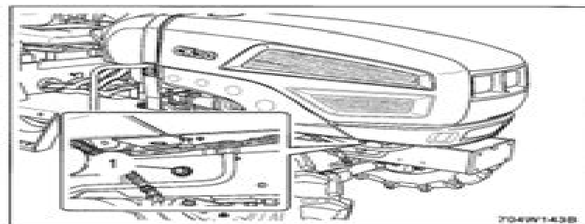
(1) Drain Plug
